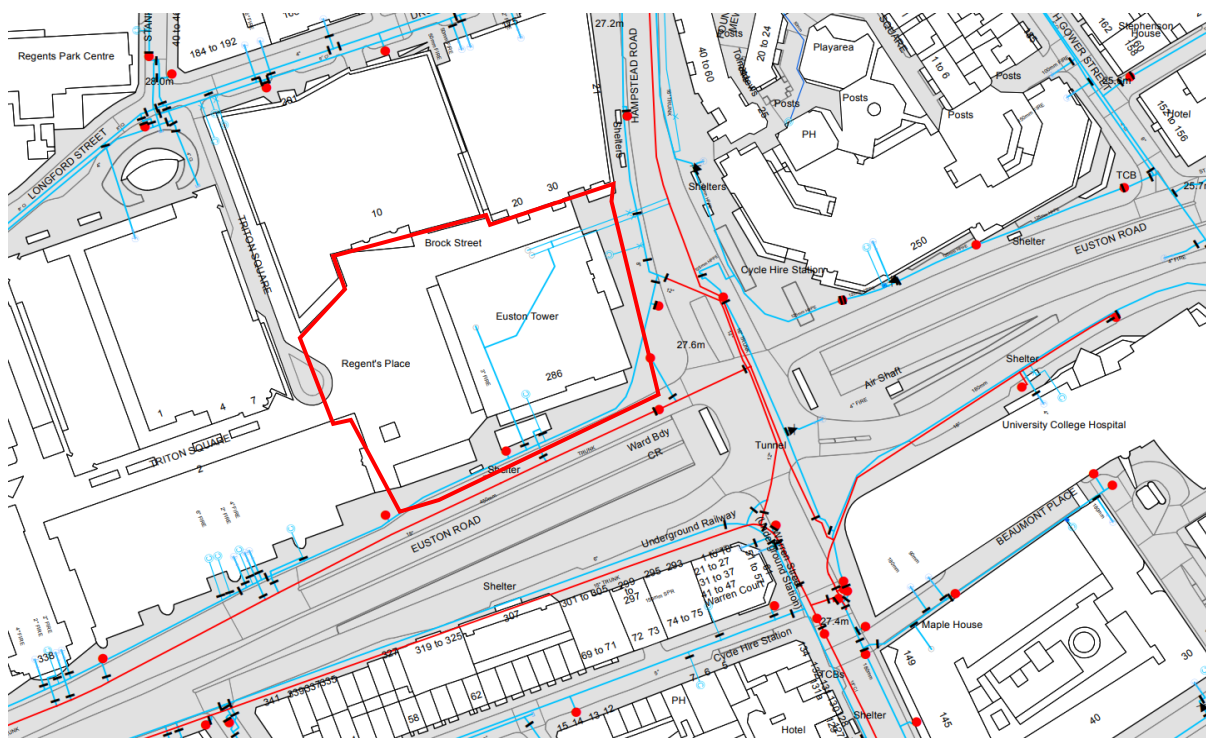
Figure 3: Existing Thames Water Potable Water Mains
