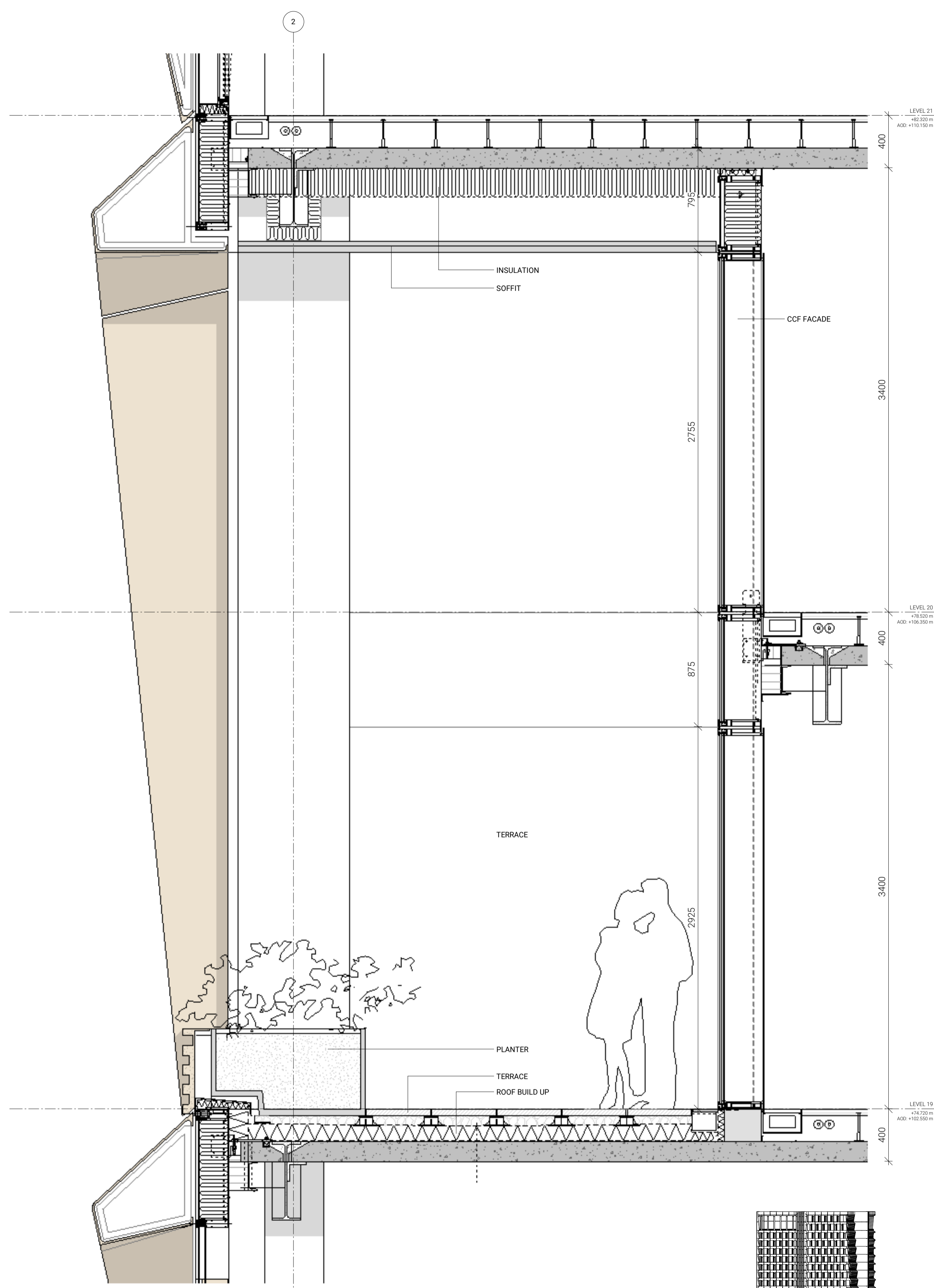
SECTION 1:20
